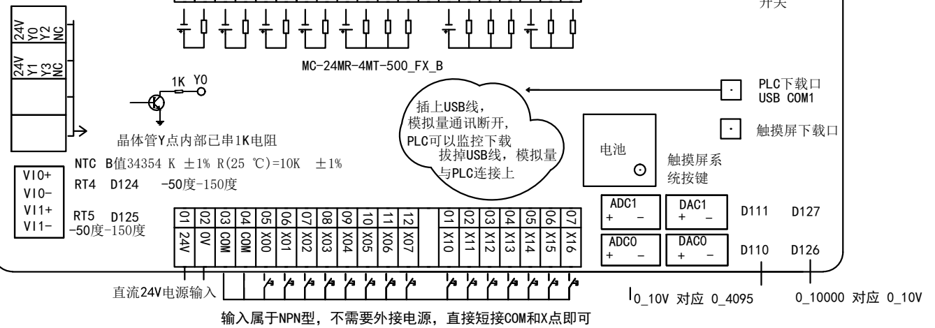
MC-24MR-4MT-500_FX_B接线图V2
